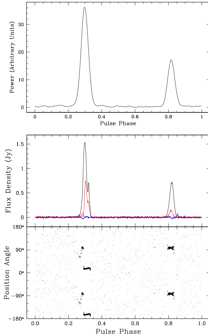
Figure 3: Pulse profile of the fastest rotating pulsar, PSR B1937+21, observed with the 76-m Lovell telescope at Jodrell Bank Observatory [67]. The top panel shows the total-intensity profile derived from a filterbank observation (see text); the true profile shape is convolved with the response of the channel filters. The lower panel shows the full-Stokes observation with a coherent dedispersion instrument [126, 123]. Total intensity is indicated by black lines, and linear and circular power by red and blue lines, respectively. The position angle of the linear polarization is plotted twice. The coherent dedispersion observation results in a much sharper and more detailed pulse profile, less contaminated by instrumental effects and more closely resembling the pulse emitted by the rotating neutron star. Much better timing precision can be obtained with these sharper pulses.
