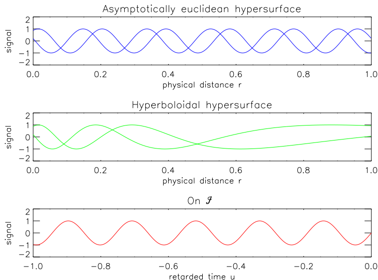
Figure 4: Wave forms in physical space-time.
