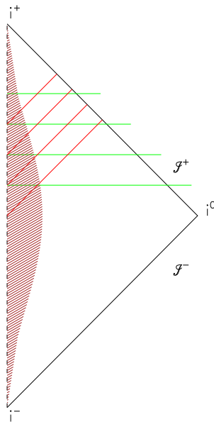
Figure 11: The geometry of the conformal approach. The green lines indicate the foliation of the conformal manifold by hyperboloidal hypersurfaces.
