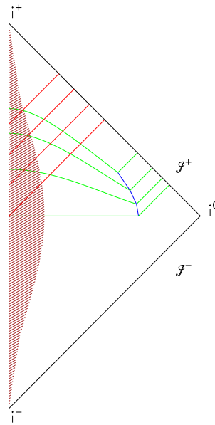
Figure 10: The geometry of Cauchy-Characteristic matching. The blue line indicates the interface between the (inner) Cauchy part and the (outer) characteristic part.
